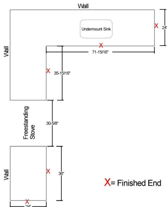
Sample Countertop Drawing
